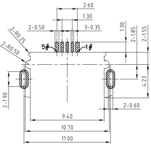
RECOMMEND PCB LAYOUT TOLERANCE: ±0.05 TOP VIEW
